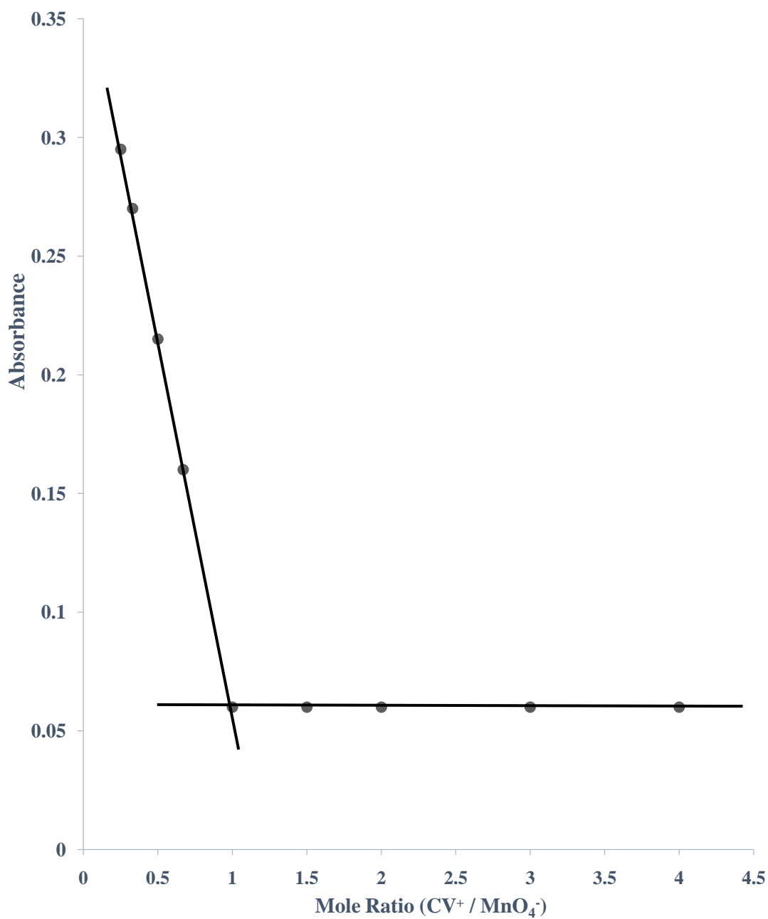
Figure 4.3: Plot of absorbance against mole ratio for the reaction of crystal violet with \text{MnO}_4^- at [\text{CV}^+] = 1.0 \times 10^{-5} \text{ mol dm}^{-3} , [\text{MnO}_4^-] = (0.25 - 4.0) \times 10^{-5} \text{ mol dm}^{-3} , [\text{H}^+] = 5 \times 10^{-2} \text{ mol dm}^{-3} , I = 0.50 \text{ mol dm}^{-3} , \lambda_{\text{max}} = 585 \text{ nm} and T = 29 \pm 1^\circ\text{C}
