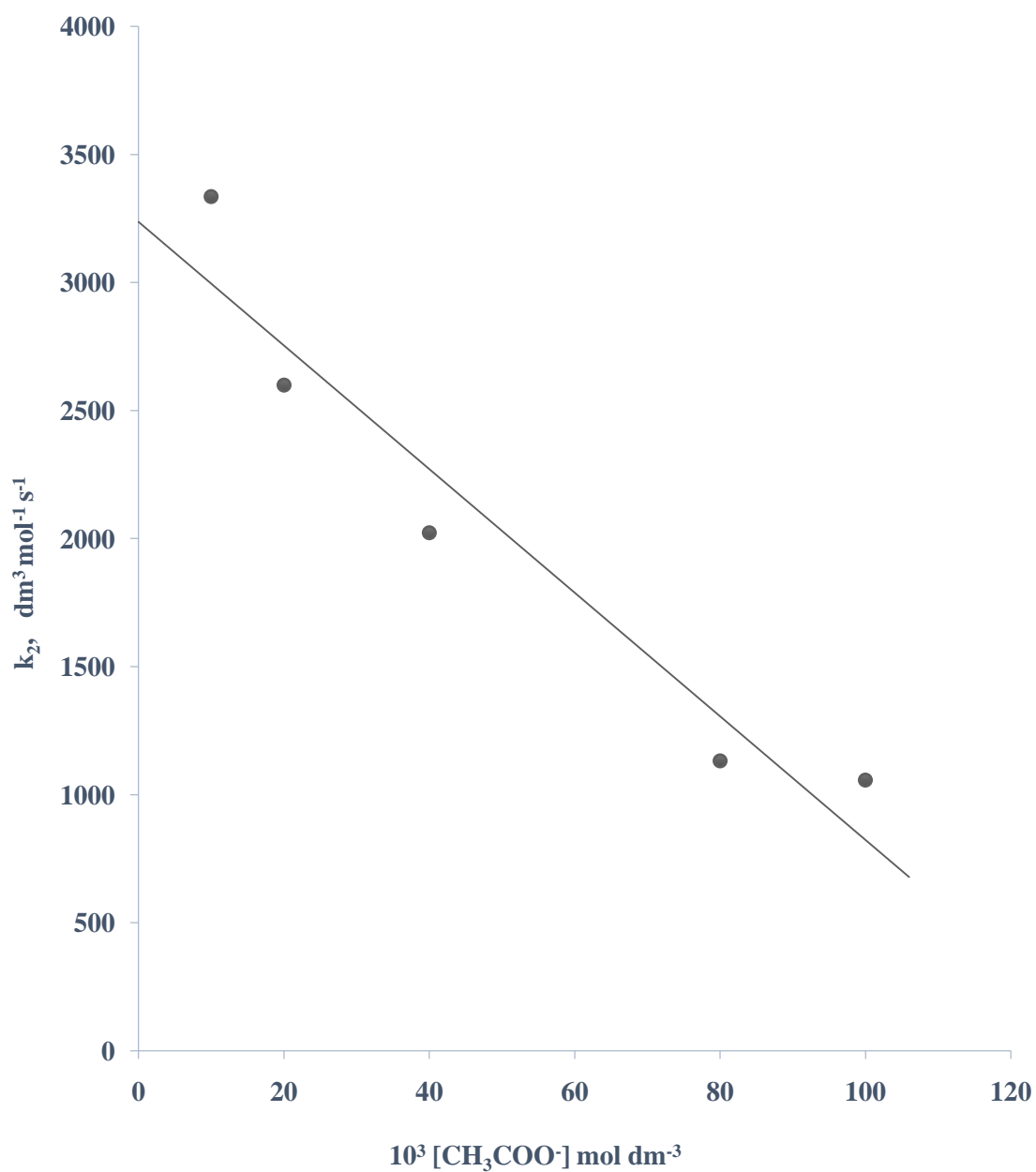
Figure 4.27: Plot of k_2 against [\text{CH}_3\text{COO}^-] for the redox reaction between crystal violet and \text{MnO}_4^- at [\text{CV}^+] = 1.0 \times 10^{-5} \text{ mol dm}^{-3} , [\text{MnO}_4^-] = 1.0 \times 10^{-4} \text{ mol dm}^{-3} , [\text{H}^+] = 5.0 \times 10^{-2} \text{ mol dm}^{-3} , [\text{CH}_3\text{COO}^-] = (10.0 - 100.0) \times 10^{-3} \text{ mol dm}^{-3} , I = 0.50 \text{ mol dm}^{-3} , \lambda_{\text{max}} = 585 \text{ nm} and T = 29 \pm 1^\circ \text{ C}
