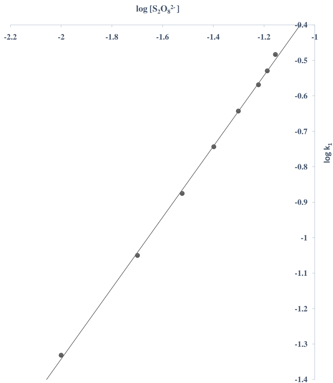
Figure 4.9: Plot of \log k_1 against \log [S_2O_8^{2-}] for the redox reaction of crystal violet with S_2O_8^{2-} at [CV^+] = 1.0 \times 10^{-5} \text{ mol dm}^{-3} , [S_2O_8^{2-}] = (1.0 - 7.0) \times 10^{-2} \text{ mol dm}^{-3} ( [H^+] = 1.0 \times 10^{-3} \text{ mol dm}^{-3} , I = 0.50 \text{ mol dm}^{-3} , \lambda_{\text{max}} = 585 \text{ nm} and T = 36 \pm 1 \text{ C} )
