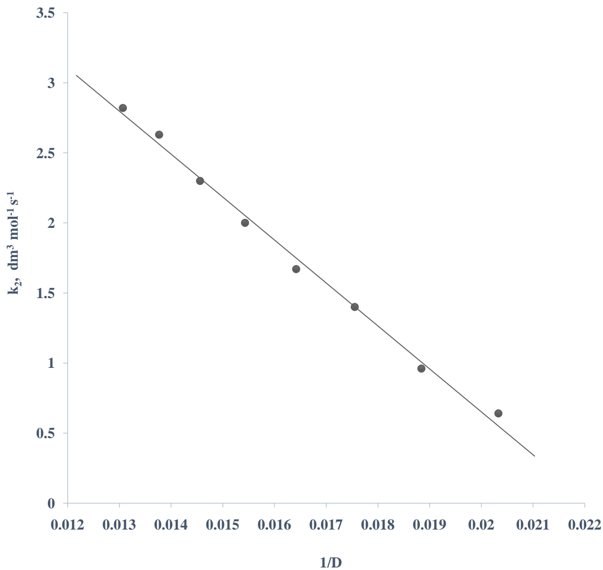
Figure 4.20: Plot of k_2 against 1/D for the redox reaction between crystal violet and S_2O_8^{2-} at [CV^+] = 1.00 \times 10^{-5} \text{ mol dm}^{-3} , [S_2O_8^{2-}] = 5.0 \times 10^{-2} \text{ mol dm}^{-3} , [H^+] = 1 \times 10^{-3} \text{ mol dm}^{-3} , I = 0.5 \text{ mol dm}^{-3} , Acetone = 10-80%, \lambda_{\text{max}} = 585 \text{ nm} and T = 36 \pm 1^\circ \text{C}
