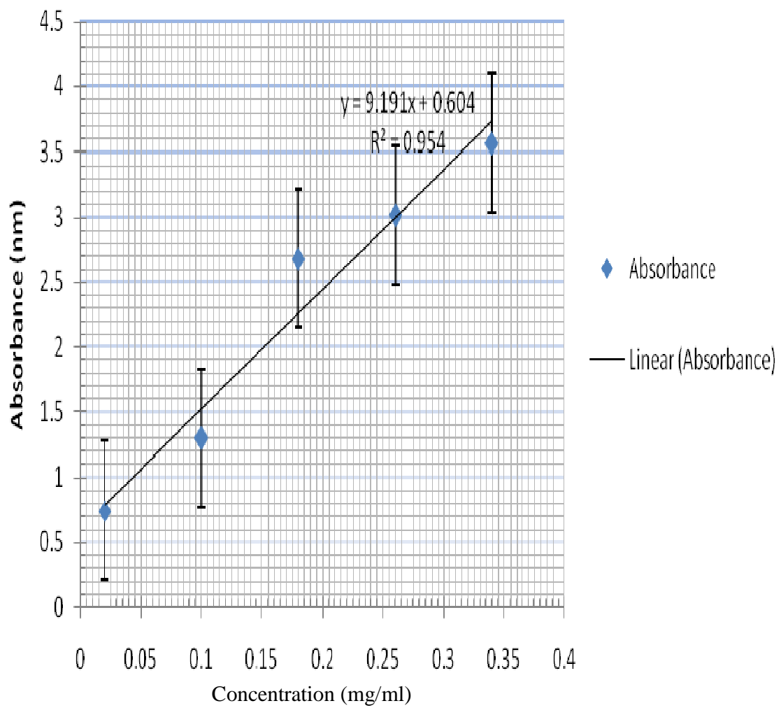
Fig15: Gallic Acid Calibration curve at 765nm
