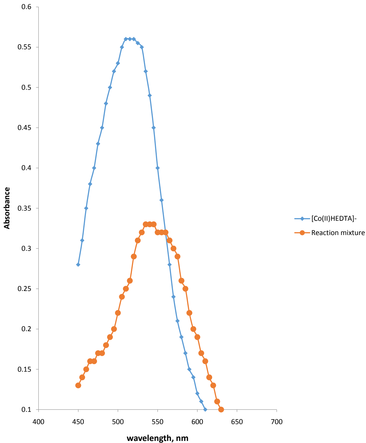
Figure 4.22: The spectrum of spectrophotometric test for the reaction of [\text{Co}^{\text{II}}\text{HEDTA}]^- with \text{S}_2\text{O}_8^{2-} at [\text{Co}^{\text{II}}\text{HEDTA}] = 5.0 \times 10^{-3} \text{ mol dm}^{-3} , [\text{S}_2\text{O}_8^{2-}] = 16.0 \times 10^{-2} \text{ mol dm}^{-3} , I = 1.0 \text{ mol dm}^{-3} , [\text{Ag}^+] = 1.0 \times 10^{-2} \text{ mol dm}^{-3} , T = 299 \pm 1\text{K} and \lambda_{\text{max}} = 525 \text{ nm}
