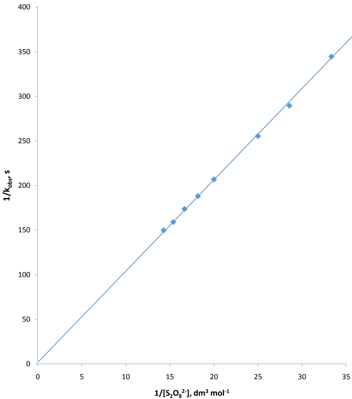
Figure 4.25: Michaelis-Menten plot for the reaction of [Co^{II}EDTA]^{2-} with S_2O_8^{2-} at [Co^{II}EDTA^{2-}] = 5.0 \times 10^{-3} mol dm^{-3} , I = 0.5 mol dm^{-3} , [Ag^+] = 1.0 \times 10^{-2} mol dm^{-3} , T = 299 \pm 1K and \lambda_{max} = 520 nm
