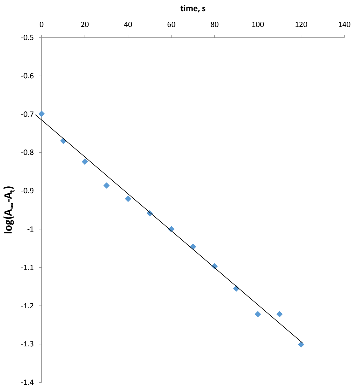
Figure 4.8: Typical pseudo-first order plot for the reaction of [\text{Co}^{\text{II}}\text{HEDTA}(\text{OH}_2)]^- with \text{ClO}^- at [\text{Co}^{\text{II}}\text{HEDTA}(\text{OH}_2)] = 5.0 \times 10^{-3} \text{ mol dm}^{-3} , \text{ClO}^- = 9.0 \times 10^{-2} \text{ mol dm}^{-3} , I = 0.2 \text{ mol dm}^{-3} , [\text{H}^+] = 1.0 \times 10^{-2} \text{ mol dm}^{-3} , T = 300 \pm 1\text{K} and \lambda_{\text{max}} = 525 \text{ nm}
