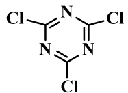
Cyanuric Chloride
