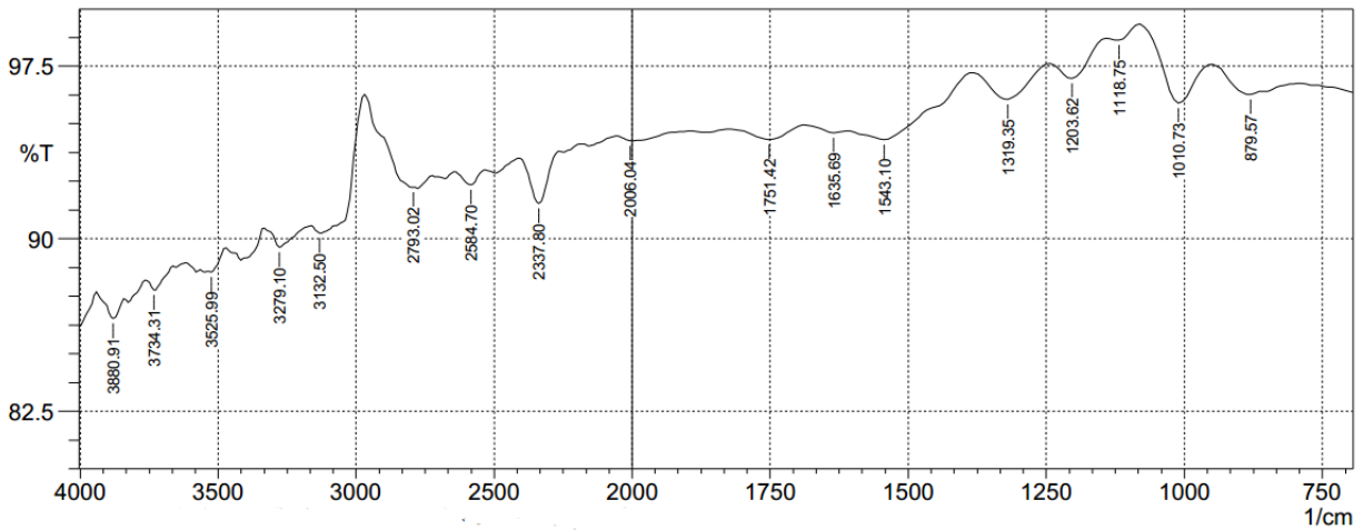
Figure A13: FTIR –spectrum of dye 3C
