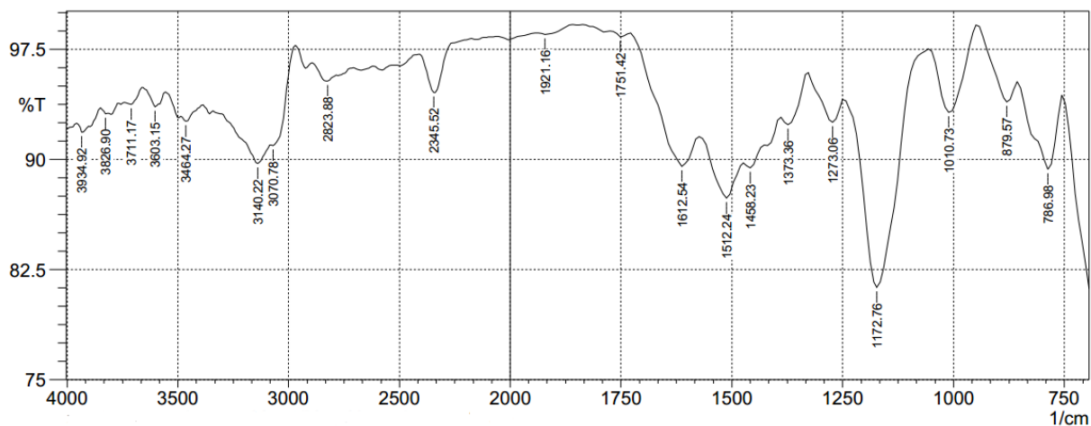
Figure A1: FTIR –spectrum of 6,7-dimethoxy-2-phenyl-4 H -benzo[ d ][1,3]oxazin-4-one
