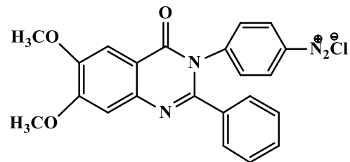
Diazonium salt
