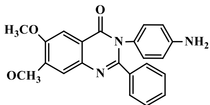
3-(4-aminophenyl)-6,7-dimethoxy-2-phenylquinazolin-4(3H)-one
