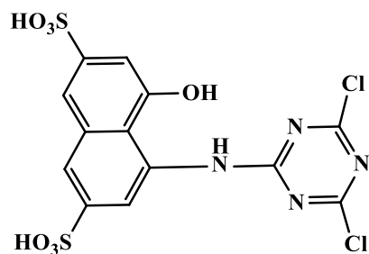
Cyanurated H-acid
