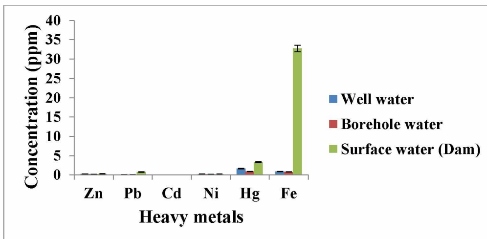
Fig. 1: Concentration of heavy metals in water samples of Bagega village in Zamfara State, Nigeria. Each bar represents mean \pm standard deviation of five (5) different samples.
