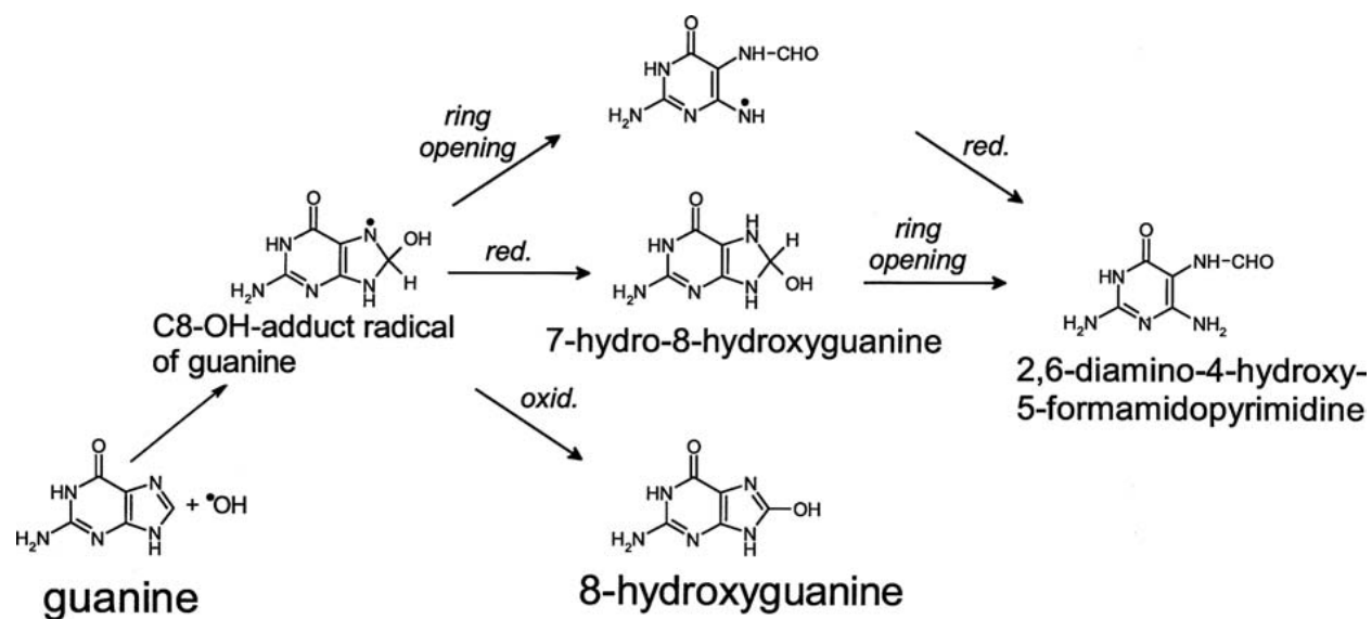
Figure 2.2 Structures of various products formed from the C8-OH-adduct radical of guanine, which itself is formed by attack of \cdot\text{OH} on the C8-position of guanine (Valko et al. , 2004)
